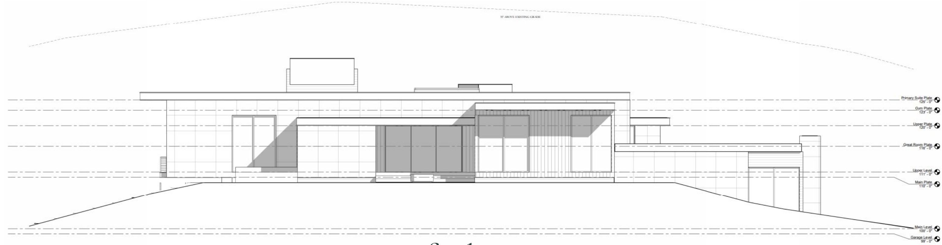
Left Elevation
